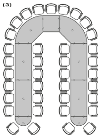
(3) 1x - 1-640 2x - 1-730 4x - 1-644 2x - 1-684 + 24x table leg
